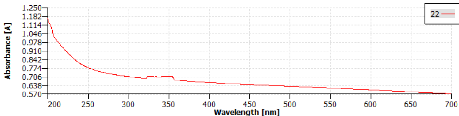
DataStream - Scan
