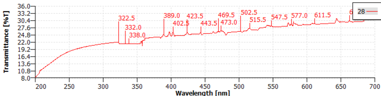
DataStream - Scan
