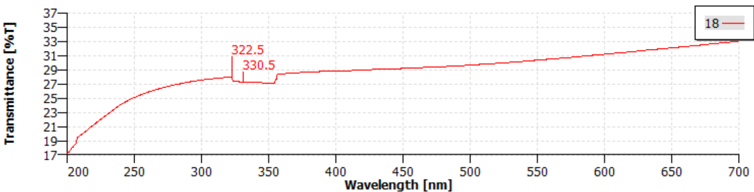
Sample Transmission
