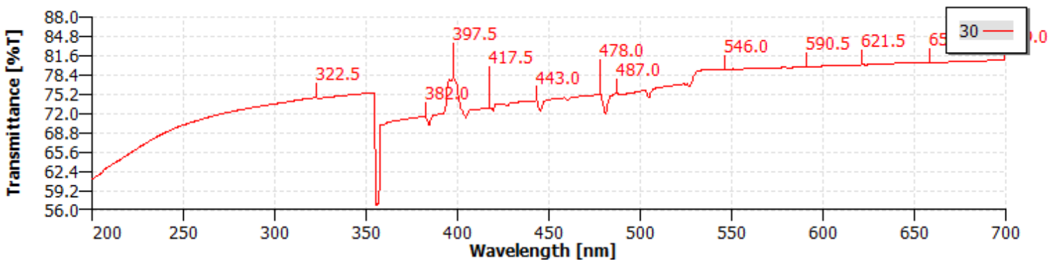
DataStream - Scan
