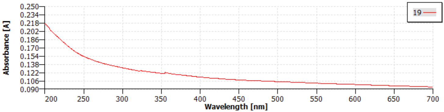
Sample Absorbance
