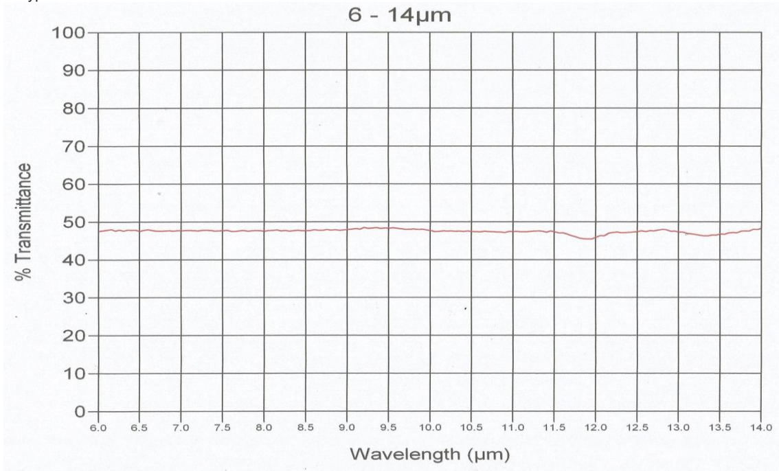
Typical transmission curve of 3mm thick
