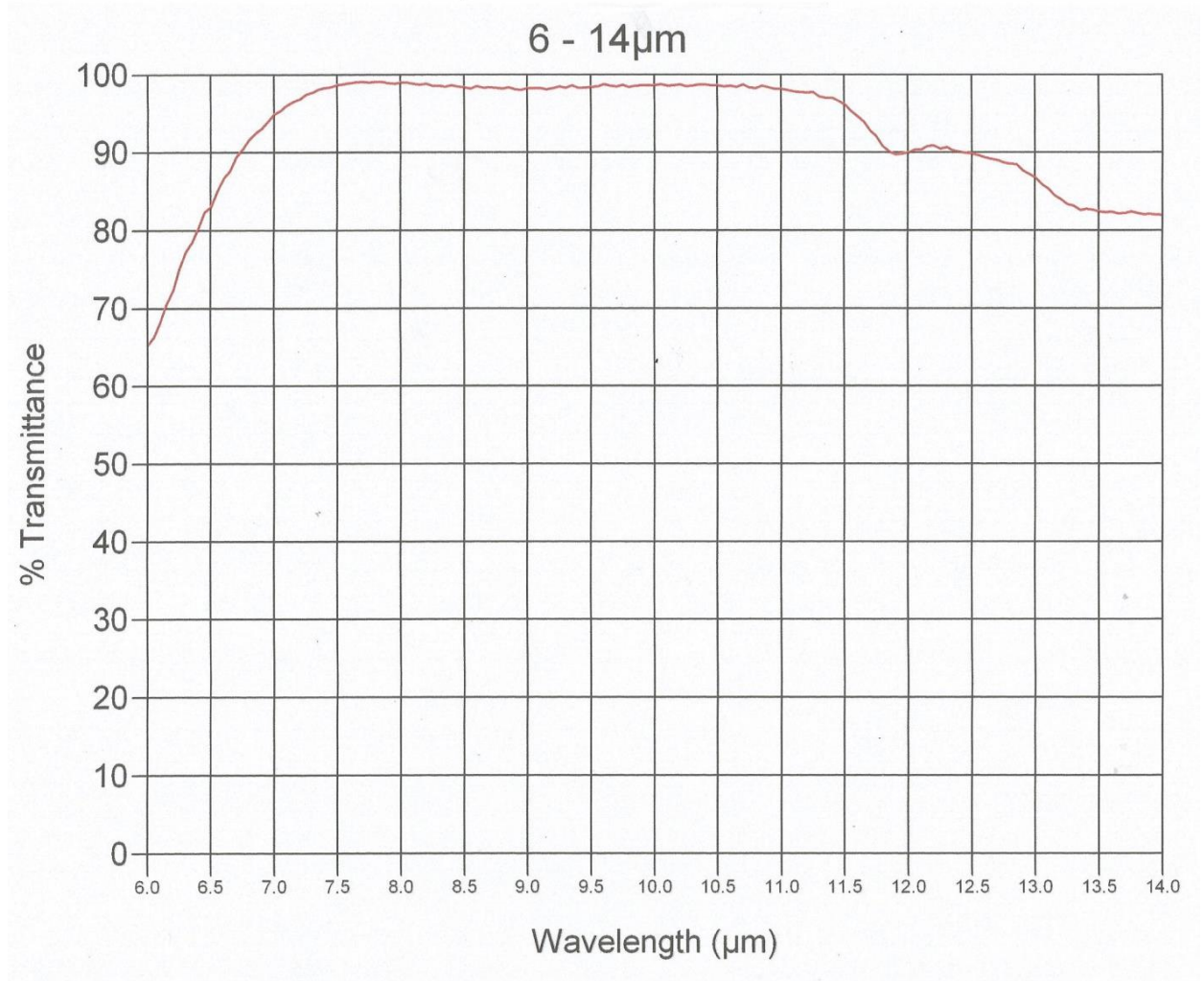
Typical Transmission 4mm thick
