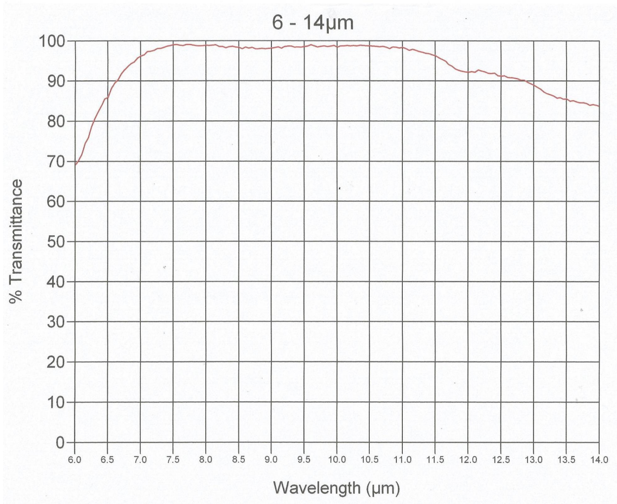
Typical Transmission 2mm thick
