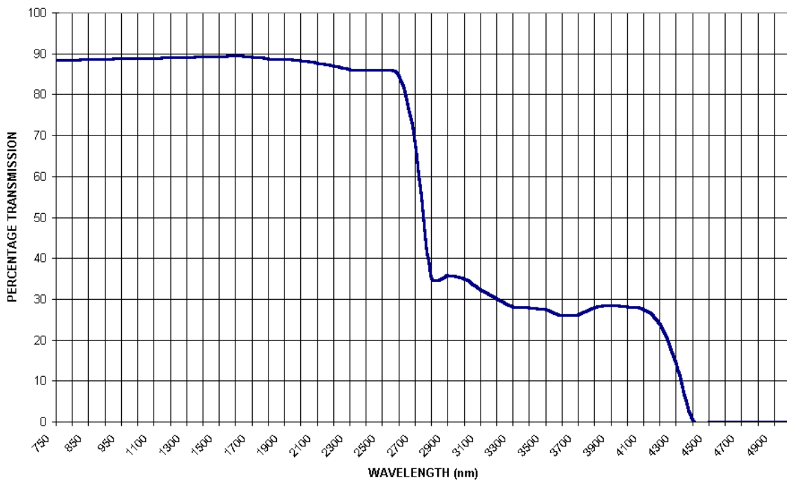
HOYA UV-34 (750 - 5000 nm)
